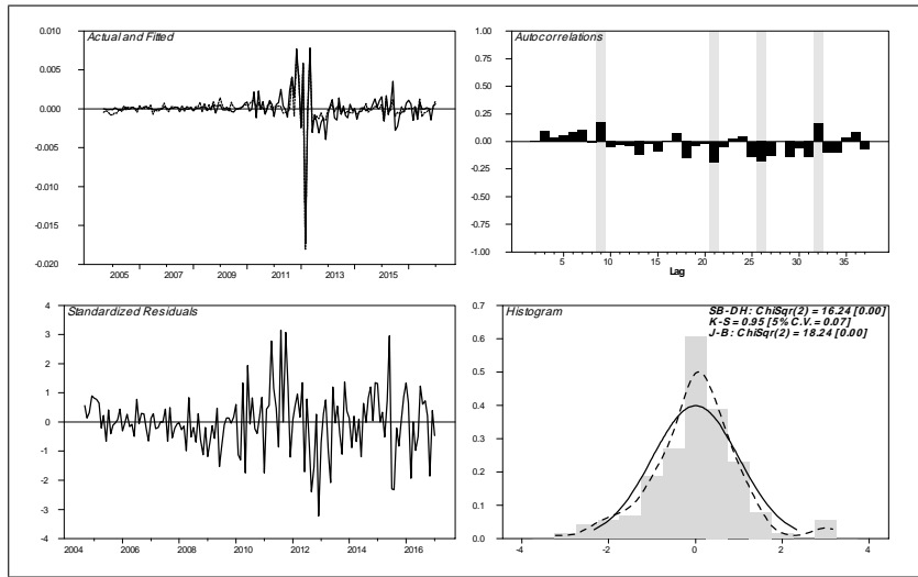
Figure 4: Graphs of actual and fitted change in the Greek bond rate (upper left hand side panel), the standardized residuals (lower left hand side panel), the residual autocorrelrogram (upper right hand side panel), and the residual histogram compared to the normal distribution.
