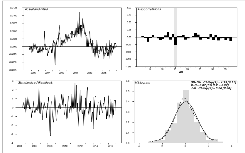
Figure 3: Graphs of actual and fitted change in the Greek unemployment rate (upper left hand side panel), the standardized residuals (lower left hand side panel), the residual autocorrelrogram (upper right hand side panel), and the residual histogram compared with the normal distribution.
