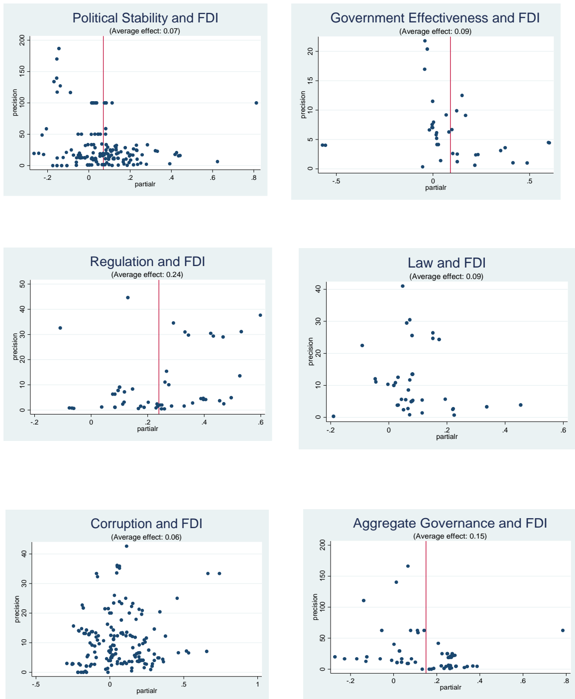
FIGURE 2.2: FUNNEL PLOTS FOR MEASURES OF GOVERNANCE AND FDI ESTIMATES 2
