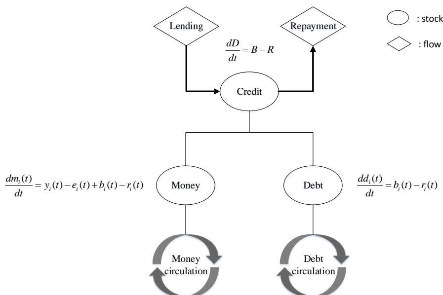
Figure 3: Flowchart of the credit creation process
