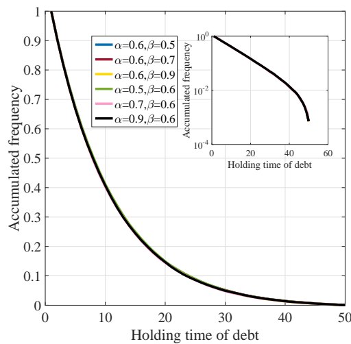
Figure 10: Holding time distribution of debt as a function of \alpha and \beta with \lambda = 0.1 , D_{max} = 10^5 . Each curve with different color represents the result for each pair of \alpha and \beta , and the inset demonstrates the same curves in the logarithmic coordinates.
