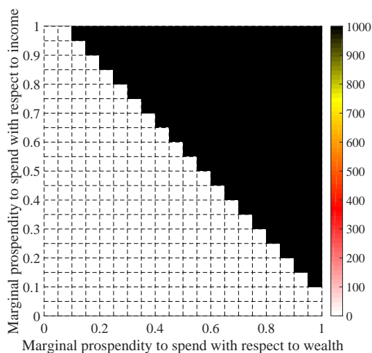
Figure 6: Number of agents who borrow as a function of \alpha and \beta with \lambda = 0.1 , D_{max} = 10^5 . The system has been separated into two areas, the white one is called no-indebtedness area while the black one is called all-indebtedness area.
