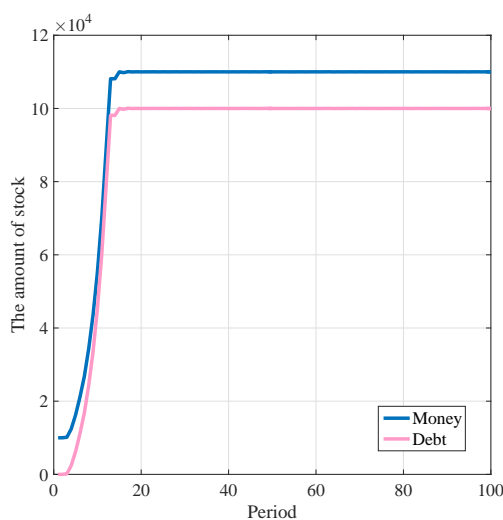
Figure 4: The evolution process of both money and debt, with \alpha = 0.5 , \beta = 0.8 , \lambda = 0.1 , D_{max} = 10^5 . The blue curve represents the evolution of money over time while the pink curve represents that of debt.
