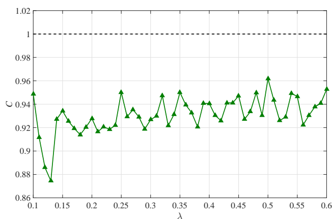
Figure 15: Ratio of realized repayment to the required repayment as a function of \lambda with \alpha = 0.8 , \beta = 0.9 and D_{max} = 10^5 . Here, c can be obtained by c = \frac{R}{\lambda D} , which is always below 1.
