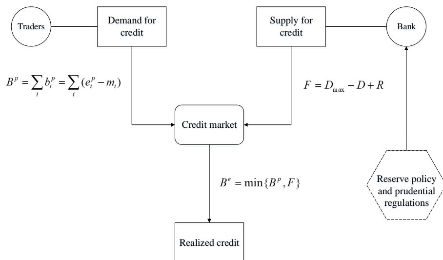
Figure 2: Flowchart of the credit transaction process
