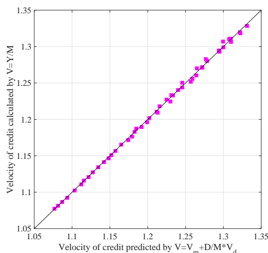
Figure 16: Comparison between two expressions of velocity with \alpha = 0.8 , \beta = 0.9 and D_{max} = 10^5 . One of the expression is that V = V_m + \frac{D}{M}V_d , taking as the horizontal value of each purple point, and the other expression is that V = \frac{Y}{M} , taking as the vertical value of each purple point.
