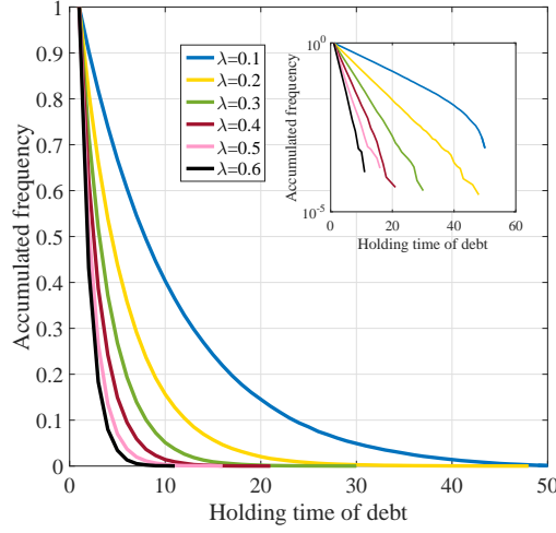
Figure 11: Holding time distribution of debt as a function of \lambda with \alpha = 0.8 , \beta = 0.9 , and D_{max} = 10^5 . Each curve with different color represents the curve for different value of \lambda , and the inset demonstrates the same curves in the semi-logarithmic coordinates.
