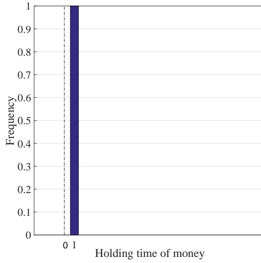
Figure 13: Holding time distribution of money with \alpha = 0.8 , \beta = 0.9 , \lambda = 0.1 and D_{max} = 10^5 . The holding time of each unit of money is equal to one.
