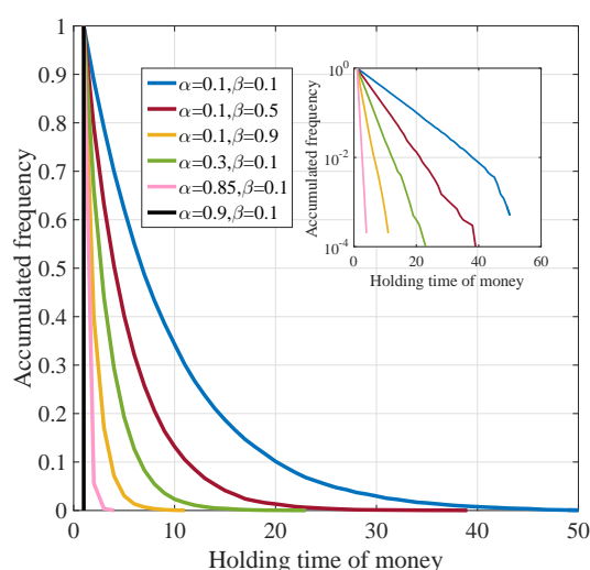
Figure 9: Holding time distribution of money as a function of \alpha and \beta with \lambda = 0.1 , D_{max} = 10^5 . Each curve with different color represents the result for each pair of \alpha and \beta , and the inset demonstrates the same curves in the semi-logarithmic coordinates.
