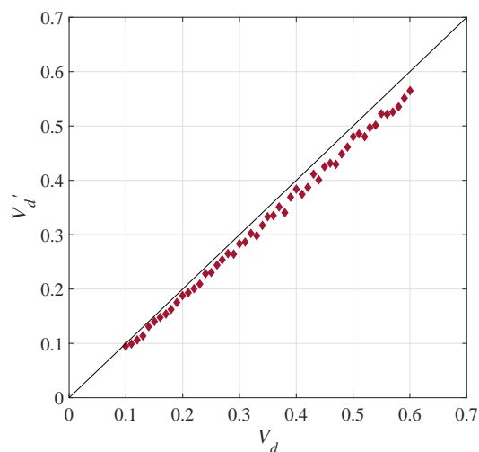
Figure 14: Comparison between theoretical results and simulation results with \alpha = 0.8 , \beta = 0.9 and D_{max} = 10^5 . V_d = \lambda , and is calculated in different values of \lambda as the horizontal value of each brown point. V'_d = \frac{1}{\bar{c}_d} , and is the expected value of holding time based on a number of simulations as the vertical value of each brown point. The dark line is the diagonal line in this coordinate.
