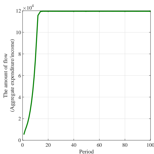
Figure 5: The evolution process of aggregate expenditure or income, with \alpha = 0.5 , \beta = 0.8 , \lambda = 0.1 , D_{max} = 10^5 . The green curve represents the evolution of aggregate expenditure or aggregate income over time.
