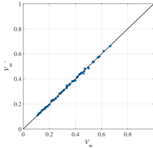
Figure 12: Comparison between theoretical results and simulation results with \lambda = 0.1 , D_{max} = 10^5 . V_m = \frac{\alpha}{1-\beta} , and is calculated in different values of \alpha and \beta as the horizontal value of each blue point. V'_m = \frac{1}{\overline{\tau}_m} , and is the expected value of holding time based on a number of simulations as the vertical value of each blue point. The dark line is the diagonal line in this coordinate.
