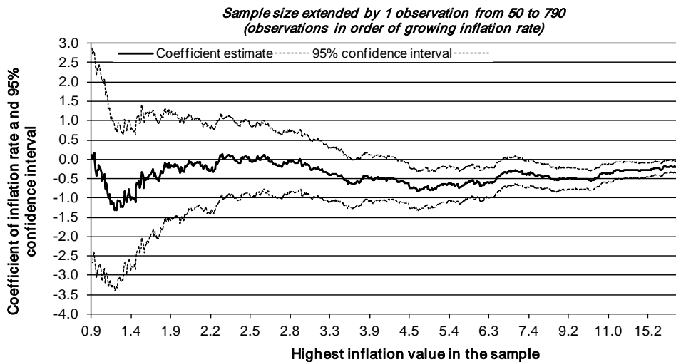
Figure 1: Coefficient of Inflation rate in Equation (1) based on the OLS Rolling Regression Estimation
